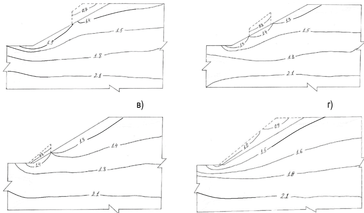
Fig. 2. Distribution of stability coefficient in the instrument array with a blade in the upper (a), middle (b), lower (c) parts and along the whole length of the slope (d).
