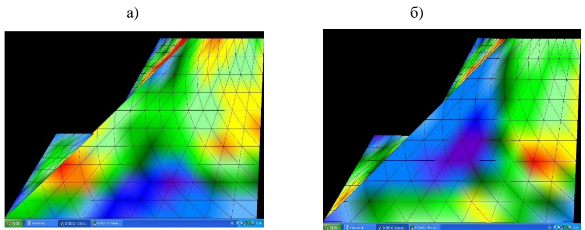
Fig. 3. Distribution of internal tensions in an instrument array at internal friction angle 300 in rocks of a file and 100 (a) and 300 (b) in rocks of a blade:
