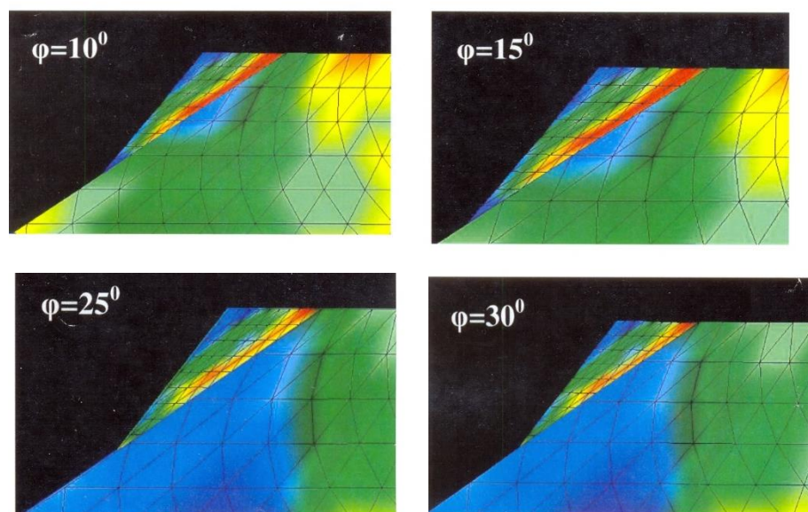
Fig.4. Distribution of internal tensions in an instrument array at constant internal friction angle in its rocks and different angles \phi in rocks of a blade (symbols on fig.4).
